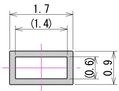
Figure 3. Example of a Recommended Nozzle Tip
